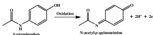
Fig. 3. Oxidation reaction of paracetamol on the surface of the graphene oxide electrode
