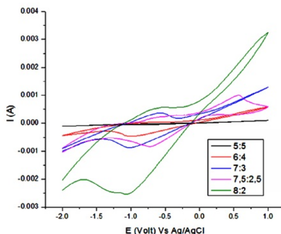
Fig. 1. Cyclic voltammogram of a 0.1 M phosphate buffer solution (pH = 6.0) containing 50 ppm of paracetamol and 5 ppm potassium chloride at various composite graphene oxides. In all the cases, the scan rate is 100 mV s -1 .
