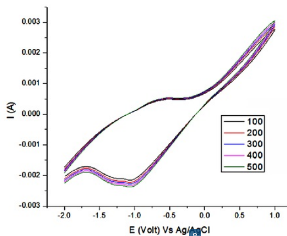
Fig. 5. Cyclic voltammogram at graphene oxide in 0.1 M phosphate buffer solution (pH = 6.0) at different scan rates. The scan rates from inner to outer are: 100 to 500 mV s -1 . The solution contains 50 ppm of paracetamol and 5000 ppm potassium chloride. In all the cases, the scan rate is 100 mV s -1 .
