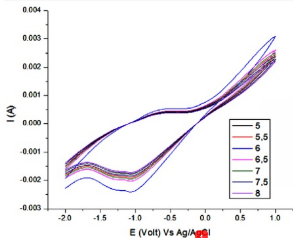
Fig. 2. Cyclic voltammogram at graphene oxide in 0.1 M phosphate buffer solution (pH = 6.0) at different pHs containing 50 ppm of paracetamol and 5000 ppm potassium chloride. In all the cases, the scan rate is 100 mV s -1 .
