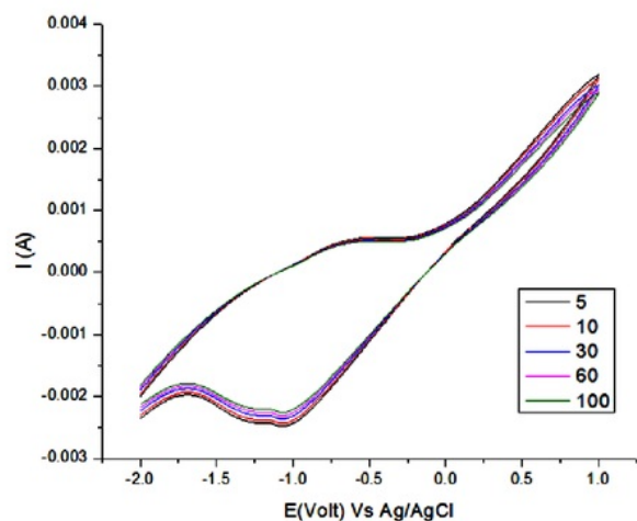
Fig. 4. Cyclic voltammogram of paracetamol 50 ppm in pH 6 buffer phosphate at scan rate of 0.1 V s -1 with various deposition time
