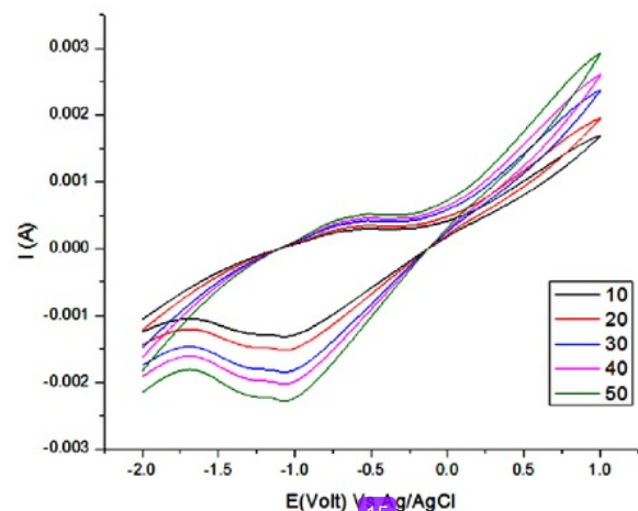
Fig. 6. Paracetamol voltamogram with a concentration of 10-50 ppm phosphate buffer solution pH 6 with a 5 s deposition time and a scan rate of 200 mV/s
